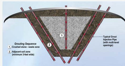
Cross-section of grout treatment zones
